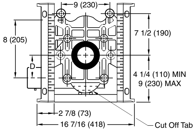
Front View SINGLE
