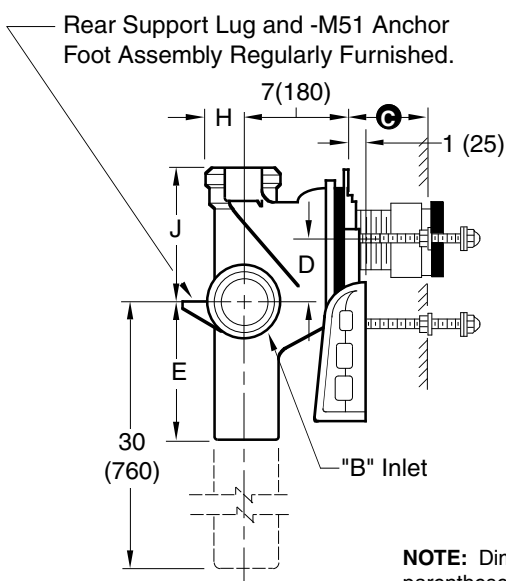
Fig. 0340L Side View
