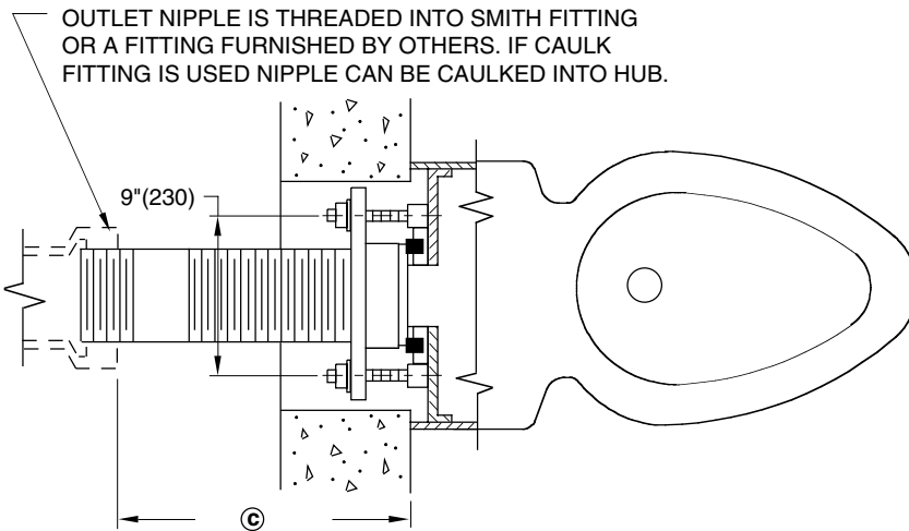
PLAN VIEW OF TYPICAL INSTALLATION
