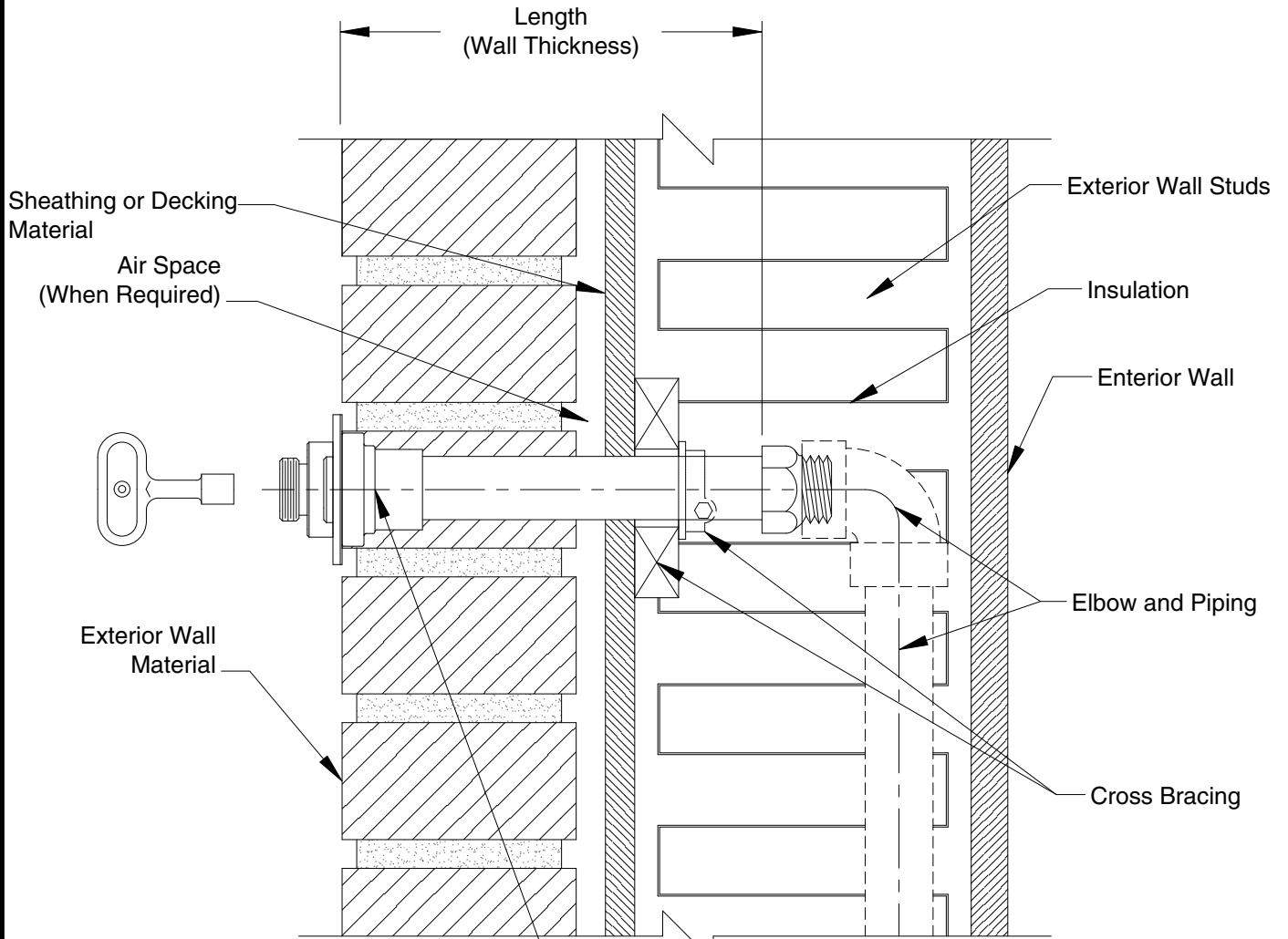
Figure 5619 Non-Freeze Hydrant Length (Wall Thickness) as Specified
