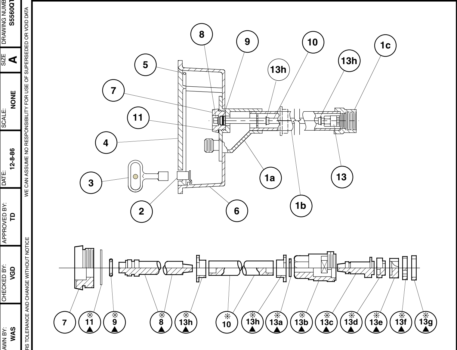
HYDRANT PARTS LIST
