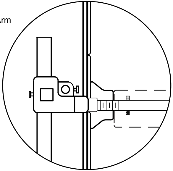
FOR JAY R. SMITH FIG. 700-E SLAB TYPE INSTALLATION
