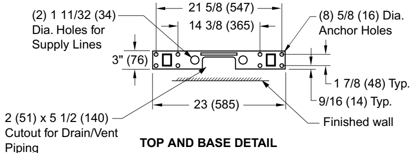
Fig. 0801D ... FOR BACK TO BACK SUPPORT
