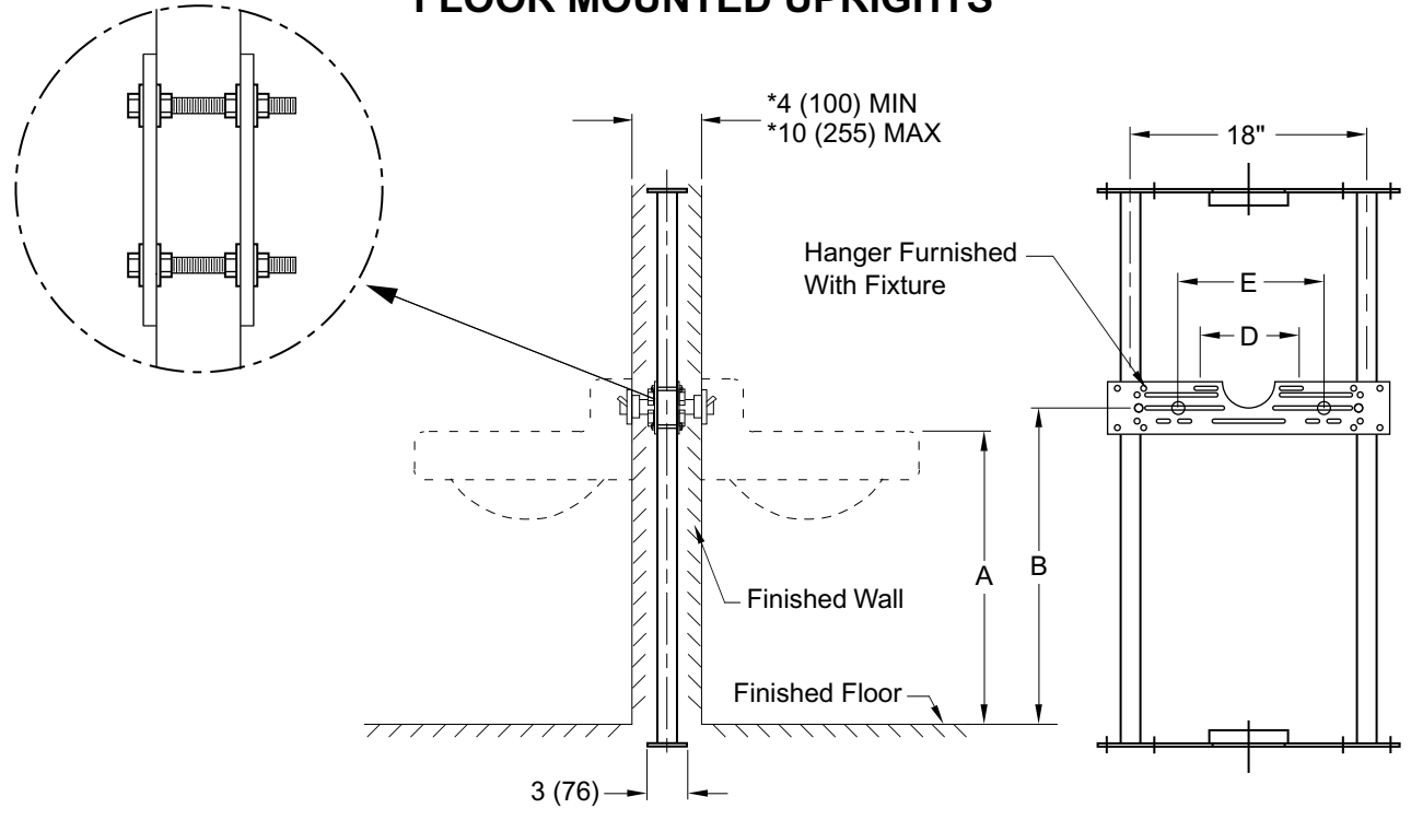
Fig. 0801D ... FOR BACK TO BACK SUPPORT
