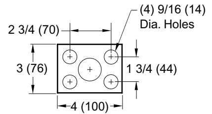
BASE DETAIL
