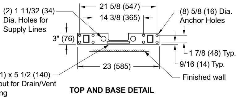
Fig. 0925 . . . WITH SUPPORTING STUDS, ADJUSTABLE COUPLING AND WASTE FITTING 4" (100) CAULK AND 4" (100) VENT FOR BACK OUTLET FLUSHING RIM SERVICE SINK
