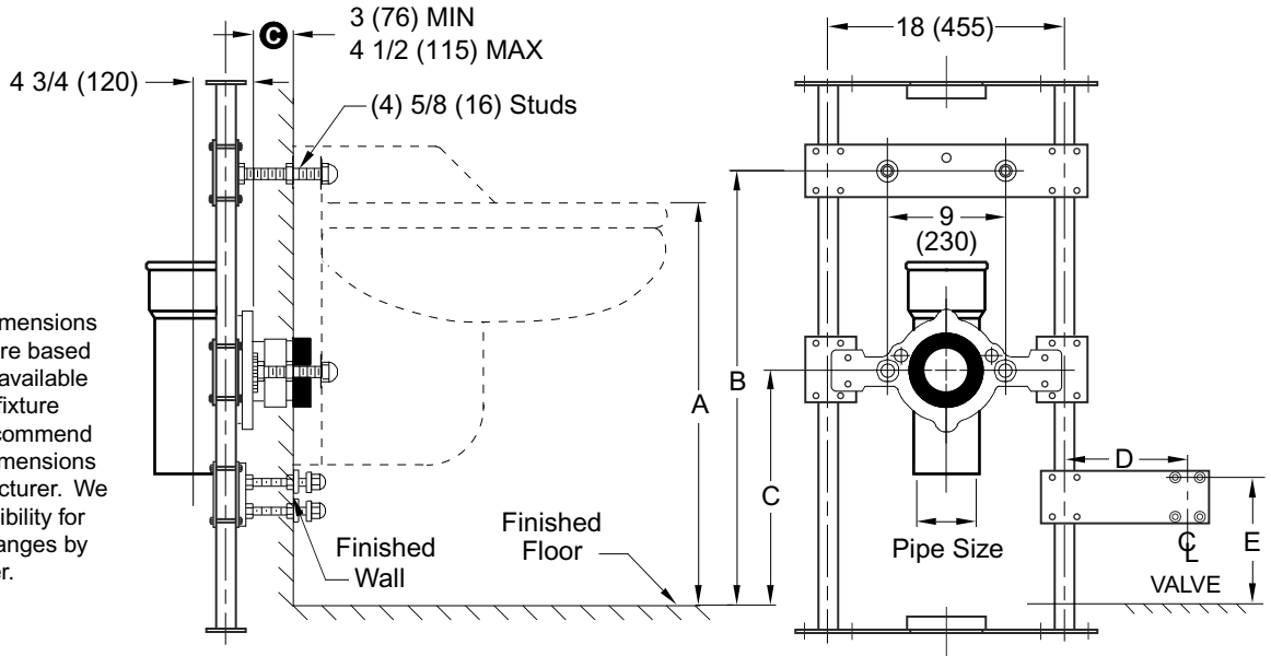
Fig. 0925 . . . WITH SUPPORTING STUDS, ADJUSTABLE COUPLING AND WASTE FITTING 4" (100) CAULK AND 4" (100) VENT FOR BACK OUTLET FLUSHING RIM SERVICE SINK
