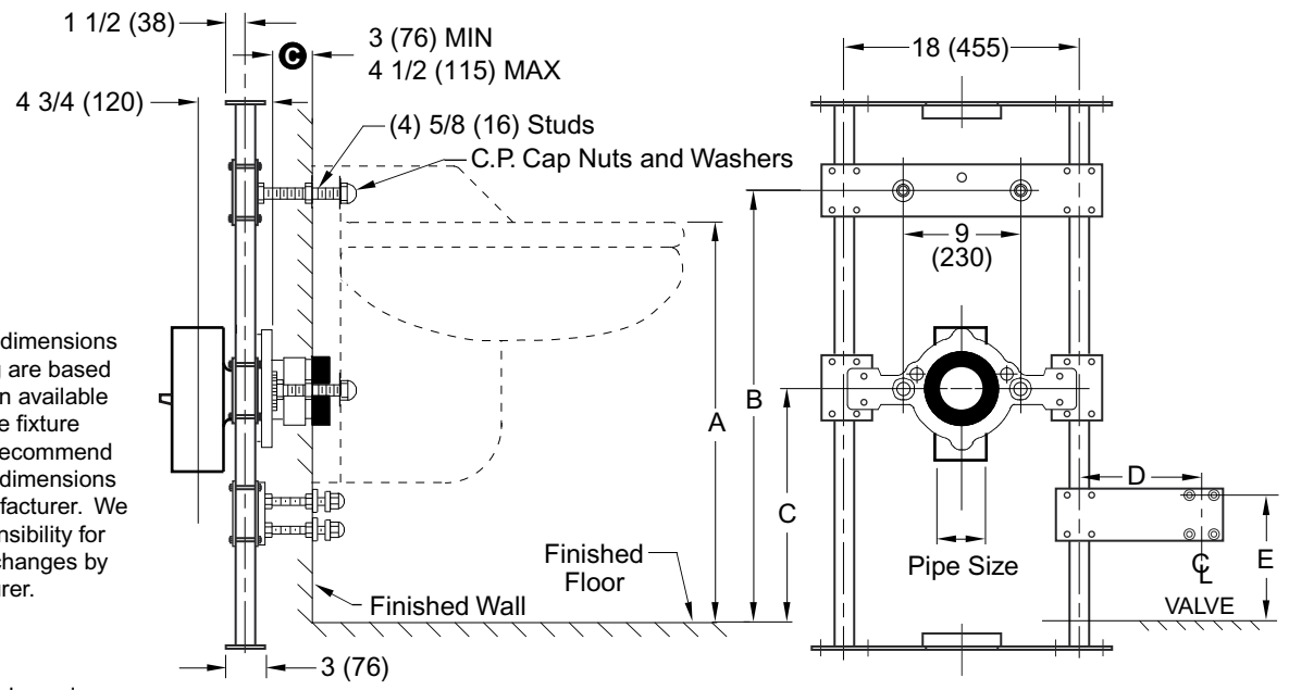
Fig. 0925 . . . WITH SUPPORTING STUDS, ADJUSTABLE COUPLING AND WASTE FITTING 4" (100) NO-HUB AND 4" (100) VENT FOR BACK OUTLET FLUSHING RIM SERVICE SINK
