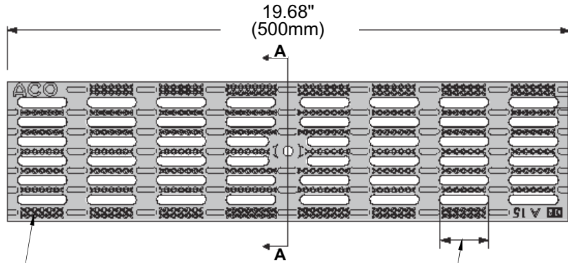
GRATE TOP VIEW
