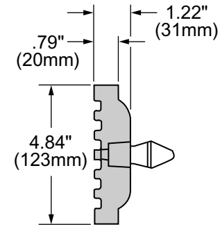
CROSS SECTION A-A
